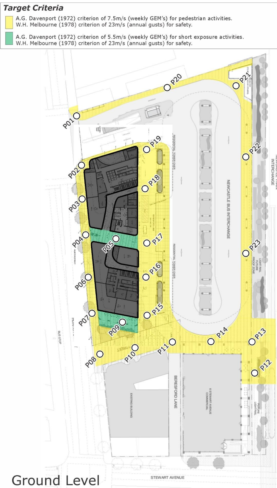
Figure 5: Study Point Locations and Target Wind Speed Criteria – Ground Floor Plan
