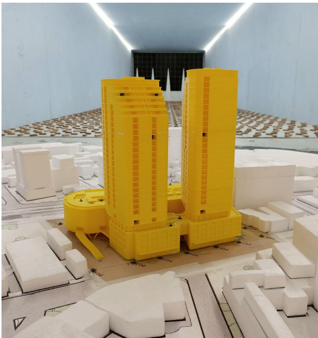
Figure 1a: Photograph of the Wind Tunnel Model (view from the south-west)
