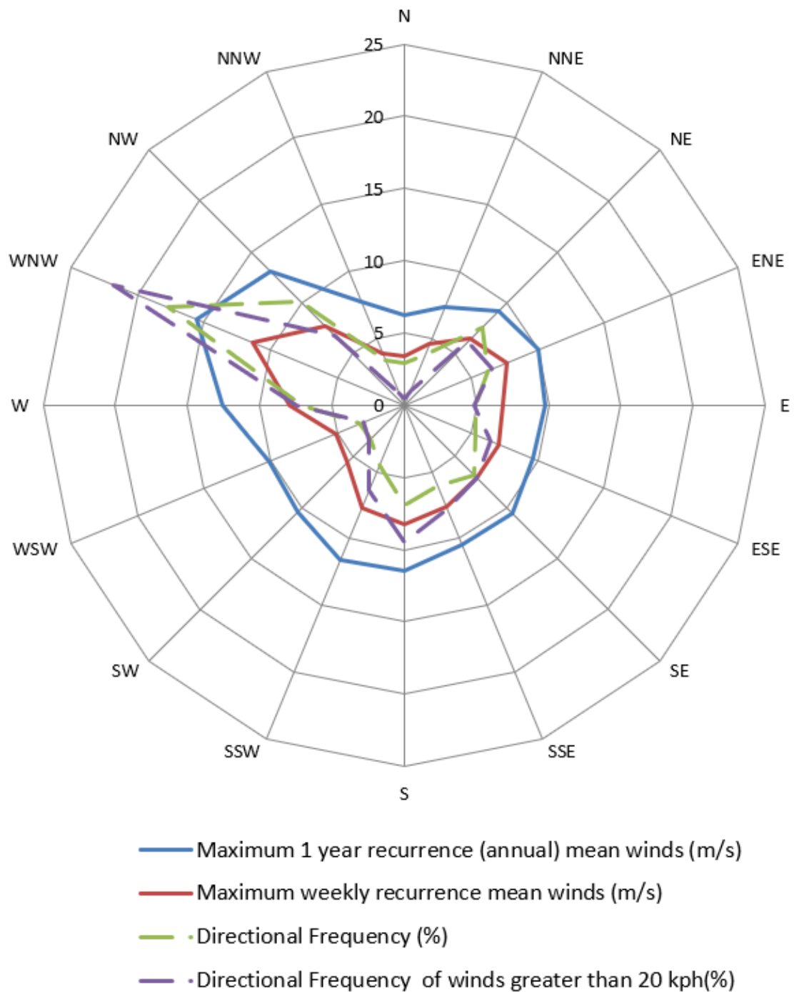
Figure 4: Annual and 5% Exceedance Hourly Mean Wind Speeds, and Frequencies of Occurrence, for the Newcastle Region (at 10m height in standard open terrain)
