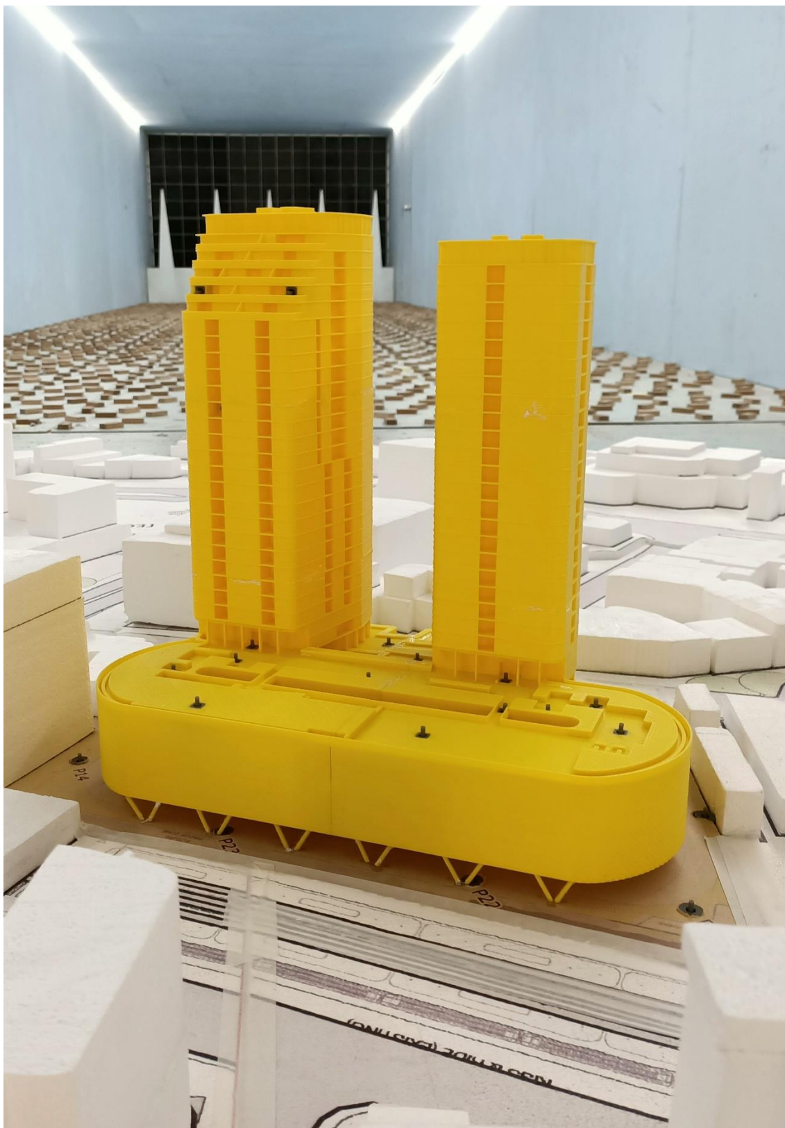
Figure 1f: Photograph of the Wind Tunnel Model (view from the north)
