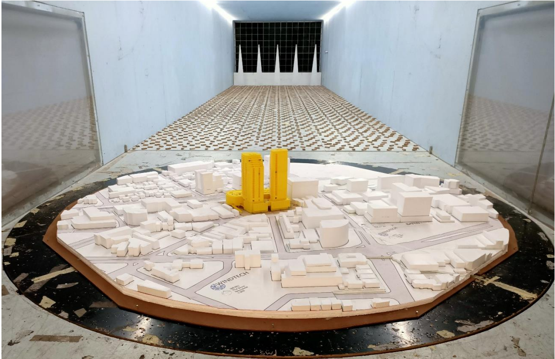
Figure 1d: Photograph of the Wind Tunnel Model (view from the south-west)
